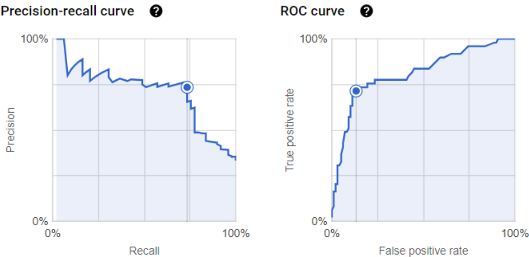
Figure 3: Evaluation metrics of a neural network trained on Vertex AI (test n=50)
